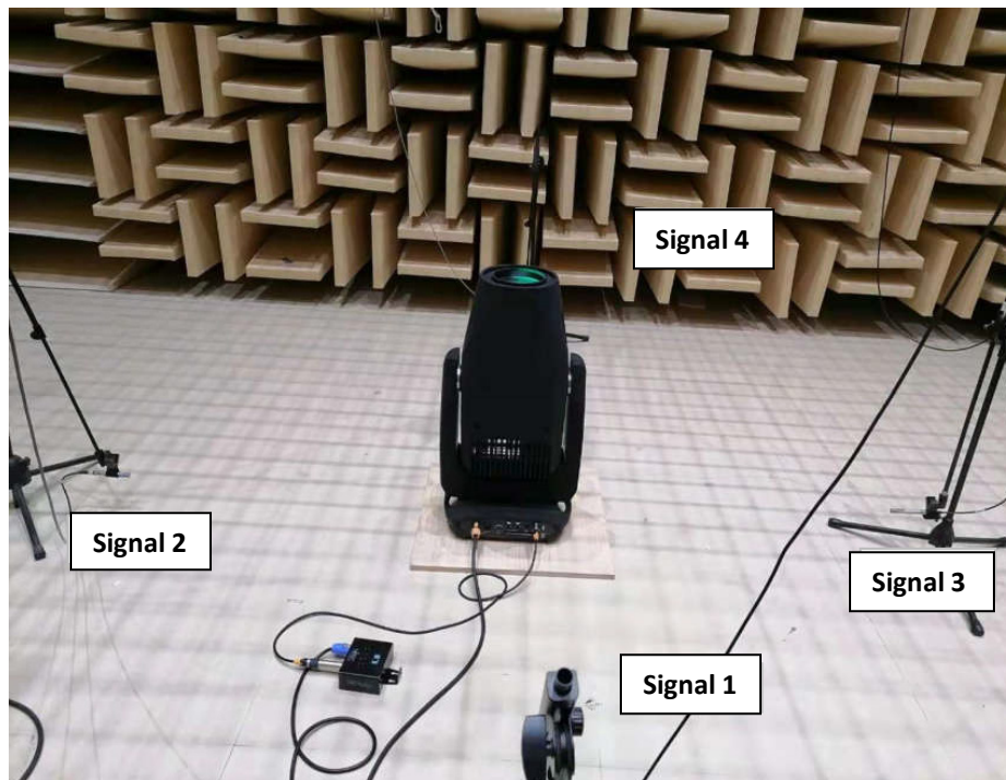
Acoustic test setup for Maverick Silens 2 Profile
