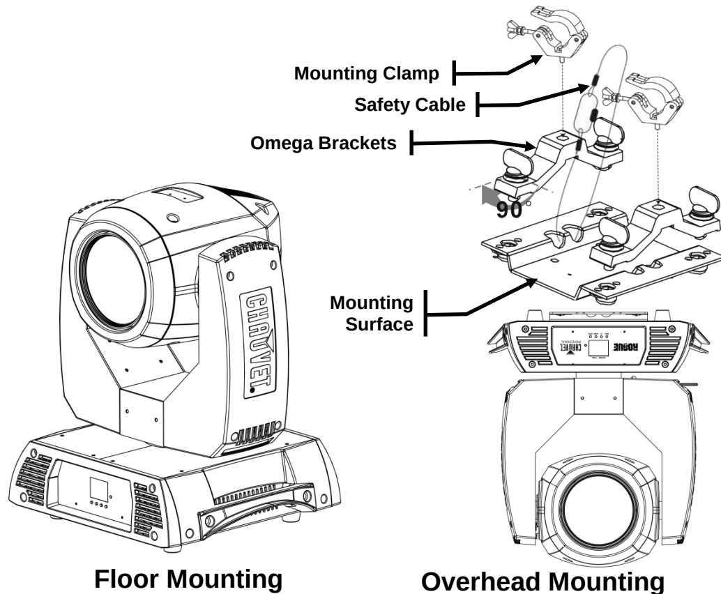
Mounting Diagram
