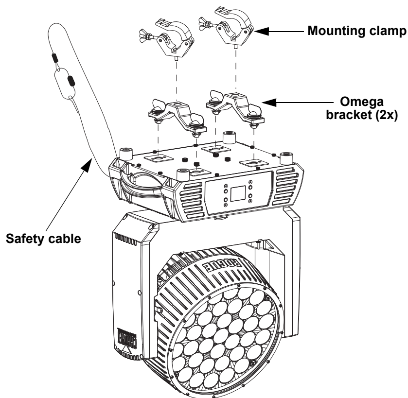
Overhead mounting
